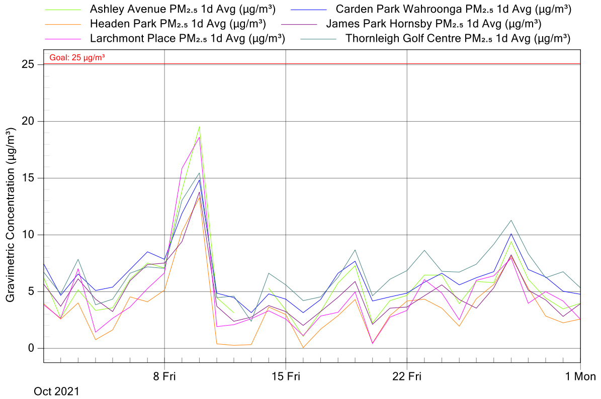
Figure 5: NorthConnex Project Air Monitoring Stations - PM 2.5 1 Day Averages for October 2021
