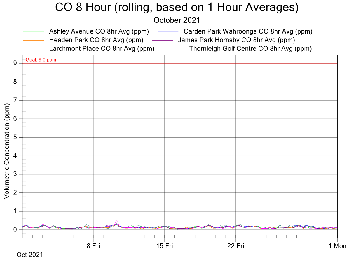
Figure 2: NorthConnex Project Air Monitoring Stations - CO 8 Hour Rolling Averages for October 2021
