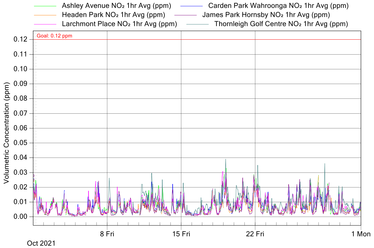
Figure 3: NorthConnex Project Air Monitoring Stations - NO 2 1 Hour Averages for October 2021
