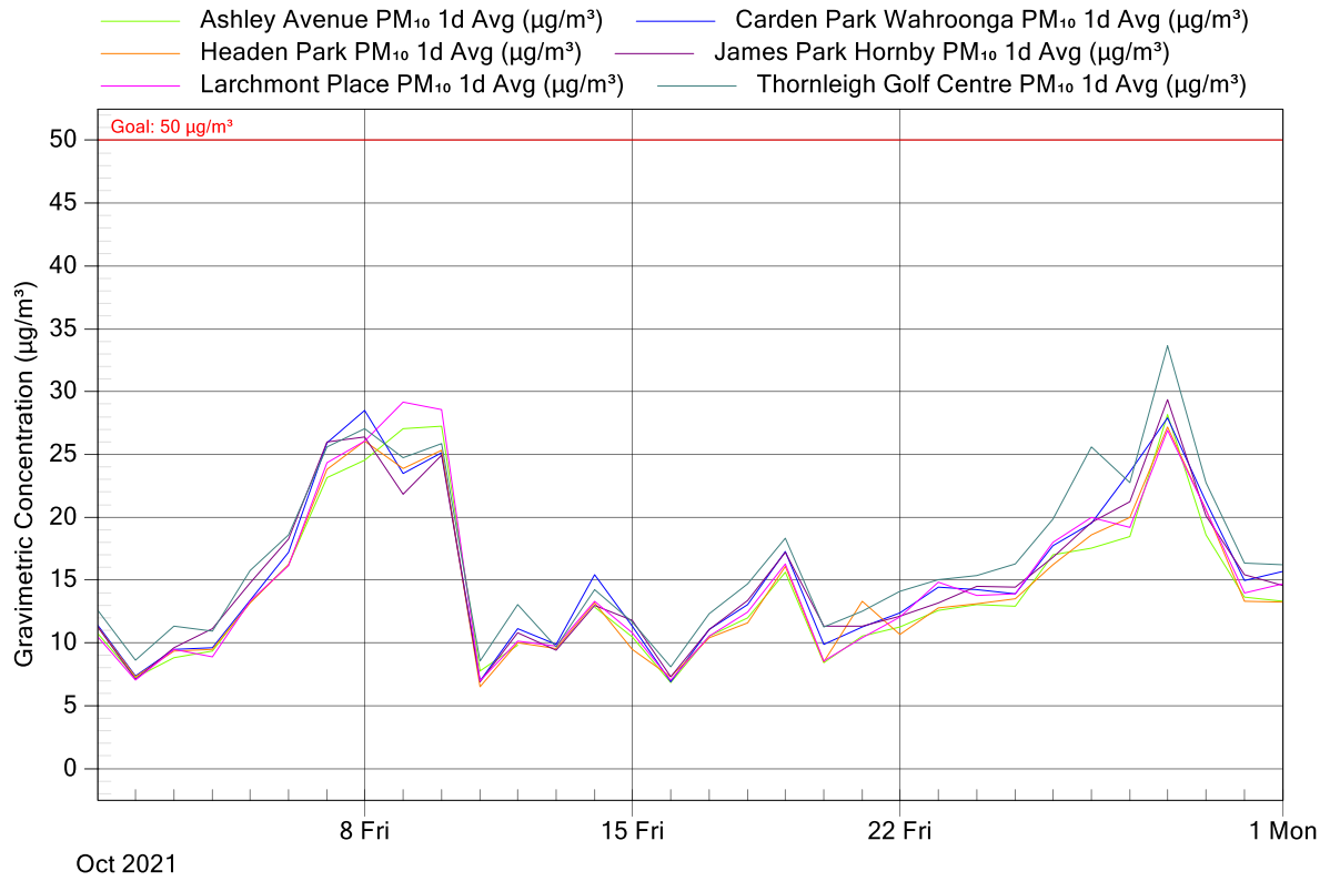
Figure 4: NorthConnex Project Air Monitoring Stations - PM 10 1 Day Averages for October 2021
